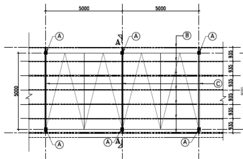
PARKING BOTTOM LEVEL PLAN
