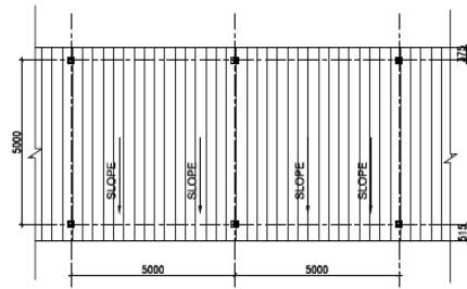
PARKING ROOF LEVEL PLAN
